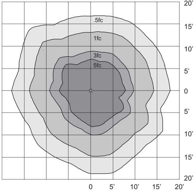
TL705 MH 100 5 IES TYPE 5 REFRACTOR
