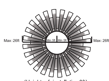
(Height of installation 8ft) Detection range
