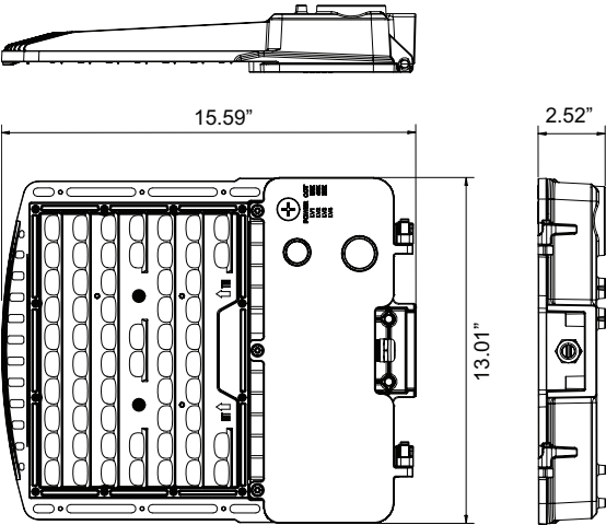
Dimensions (100/140W)
