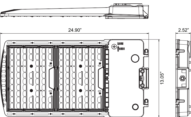
Dimensions (250/300/400W)
