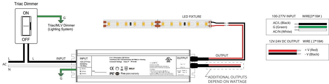
Fig. 12 - TRIAC Dimming (MLV Load Type)
