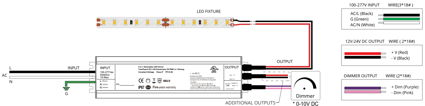
Fig. 14 - 0/1-10V Dimming
