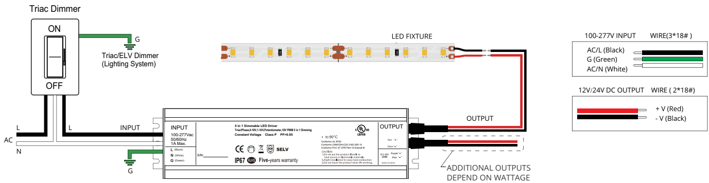
Fig. 13 - TRIAC Dimming (ELV Load Type)
