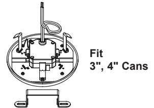
Fit 3", 4" Cans Snap-in Mounting Bracket Over A Plastic Or Metal 4/0 J-box
